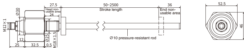
Connector external dimensions (customized type)
